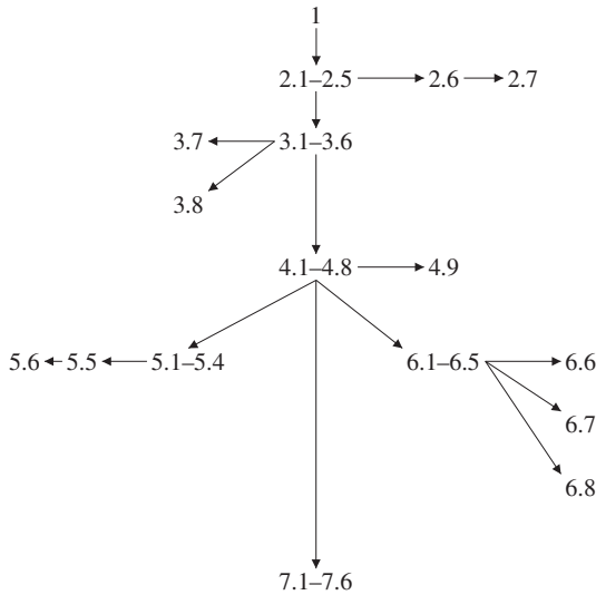
Fig. 1. Dependency Diagram
